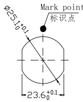
Panel cut-outs 建议安装开孔尺寸
