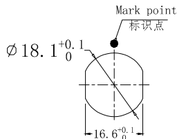
Panel cut-outs 建议安装开孔尺寸
