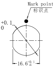
Panel cut-outs 建议安装开孔尺寸
