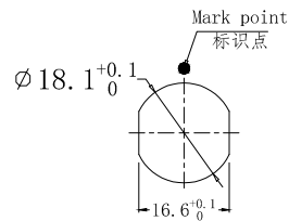
Panel cut-outs 建议安装开孔尺寸
