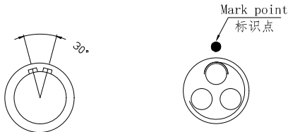
Socket front view 插座前视图
