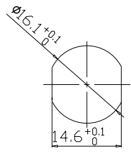
Panel cut-outs 面板开孔尺寸
