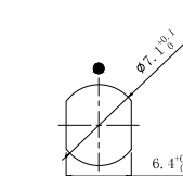
Panel cut-outs 建议安装开孔尺寸
