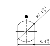
Panel cut-outs 建议安装开孔尺寸
