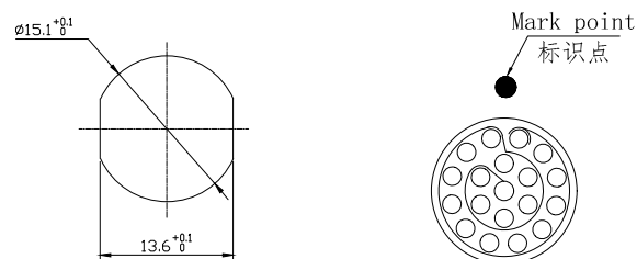
view K K向孔位排列
