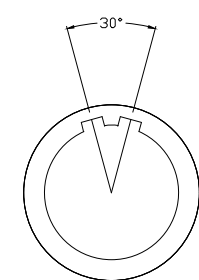
Socket front view 插座前视图
