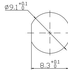
Panel cut-outs 建议安装开孔尺寸
