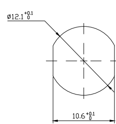
Panel cut-outs 建议安装开孔尺寸
