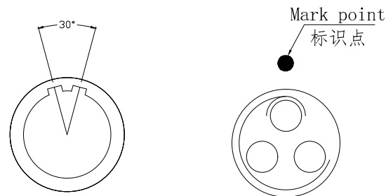
Socket front view 插座前视图
