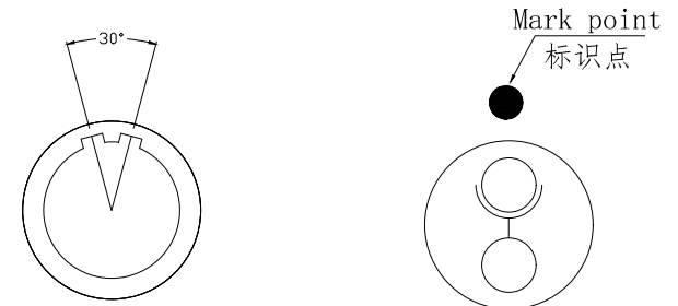
Socket front view 插座前视图
