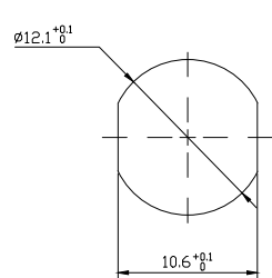
Panel cut-outs 建议安装开孔尺寸
