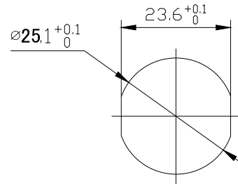
Panel cut-outs 建议安装开孔尺寸
