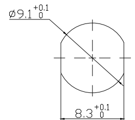
Panel cut-outs 建议安装开孔尺寸
