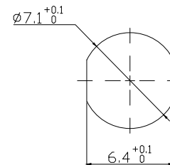
Panel cut-outs 建议安装开孔尺寸
